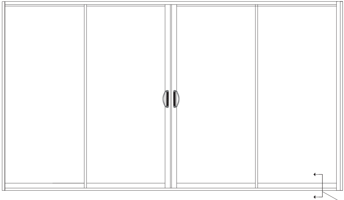
OXXO with Flat Sill
